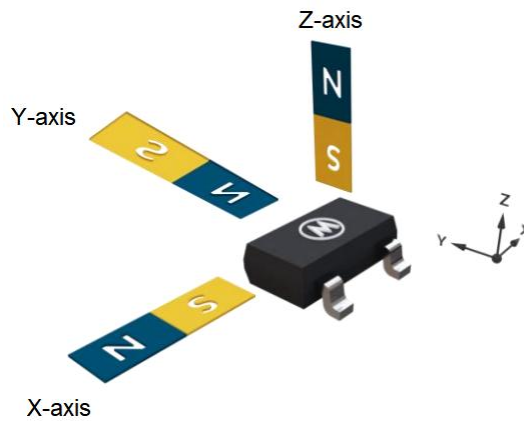
Fig 4A, 3D (X/Y/Z-Axis) Magnetic Operation of AS1190C
