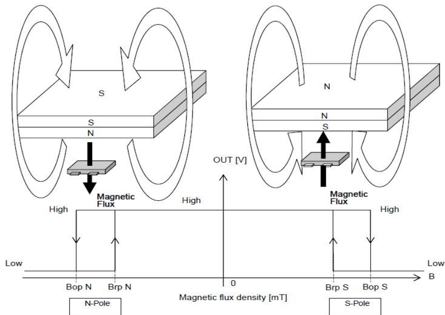
Fig 4B, Z-Axis Magnetic Operation Characteristic of AS1190C
