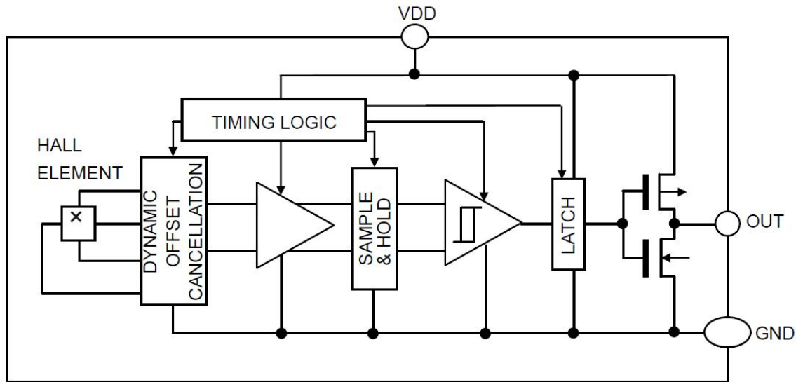
Figure 3, Block Diagram of AS1190C
