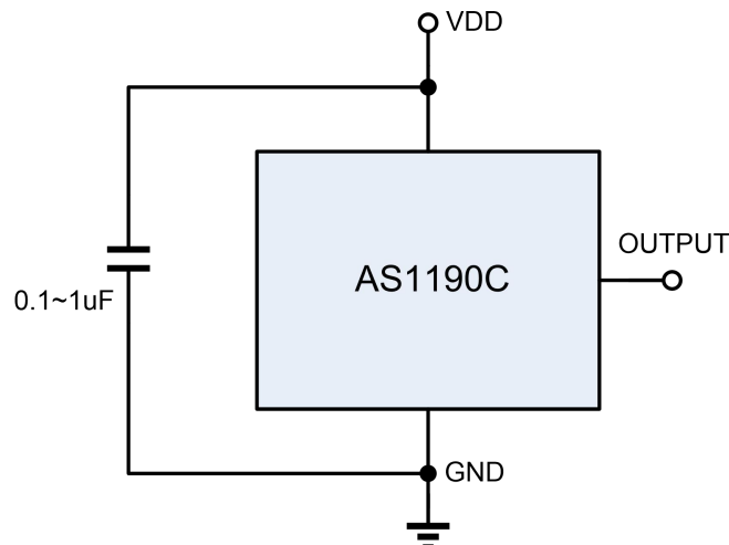
Figure 1, Typical Application Circuit of AS1190C
